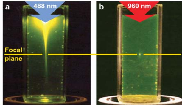
One-photon Two-photon
