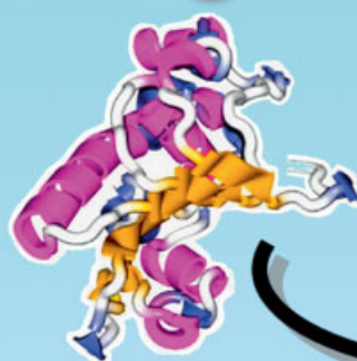
Poly(aspartate) hydrolase-1
