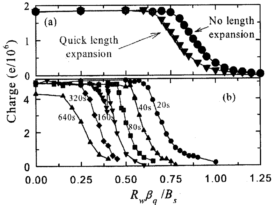
FIGURE 2. (a) Charge remaining in the trap as a function of the quadrupolar field. The “No length expansion” plasma was stored in a single cylinder of length 1 cm. The “Quick length expansion” plasma was briefly lengthened from 1 cm. to 4.08 cm. while the quadrupole was at full strength. (b) Charge remaining at the indicated times as a function of the quadrupole field. The trap length was 2 cm. The solenoidal field was 0.4 T for both (a) and (b). R_w \beta_q is the field at the trap wall.
