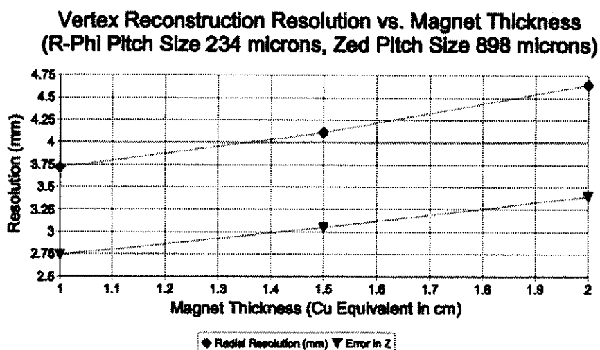
FIGURE 5. Results of the Monte Carlo simulation using the geometry shown in fig. 4 whilst varying the thickness of scattering material.
